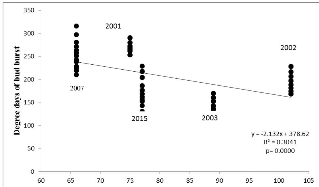
Figure 28: Number of days below 5°C between November 1 and March 1
